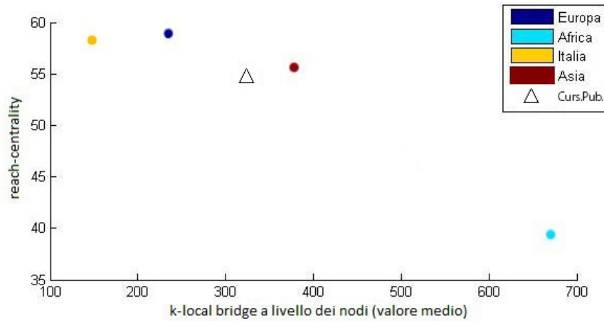
Figure 6: k-local bridge (x-axis) vs reach centrality (y-axis). The Italian and the European network form together the most efficient and robust road systems, since they both maximize the reach-centrality, while keeping the k-local bridge reasonably low.
